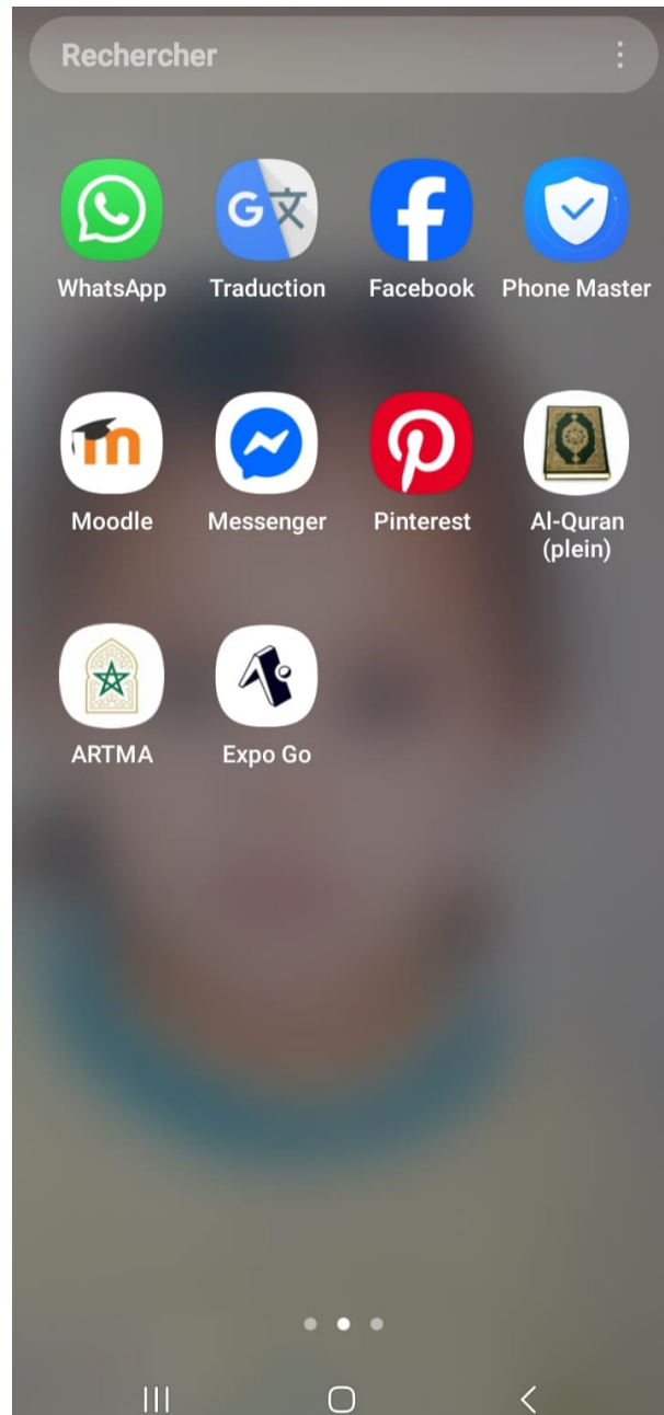
FIGURE 7 – Application installé
