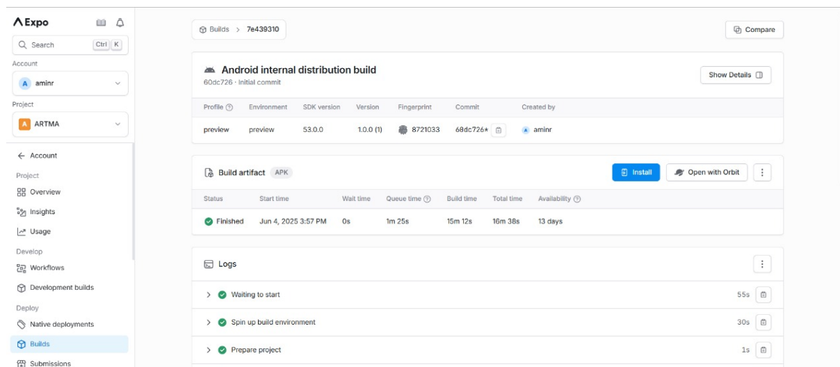
FIGURE 6 – APK
